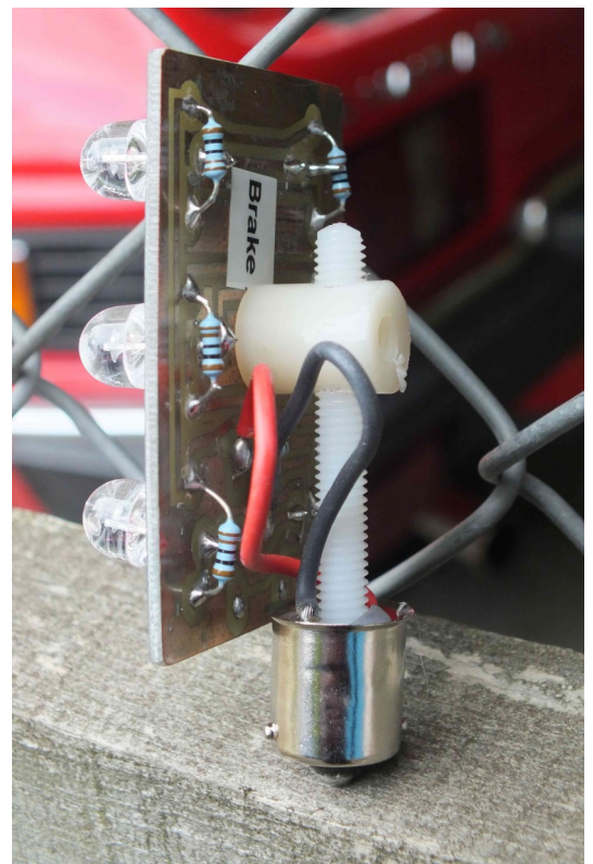
Right: Light board showing detail of adjuster and lamp base.
